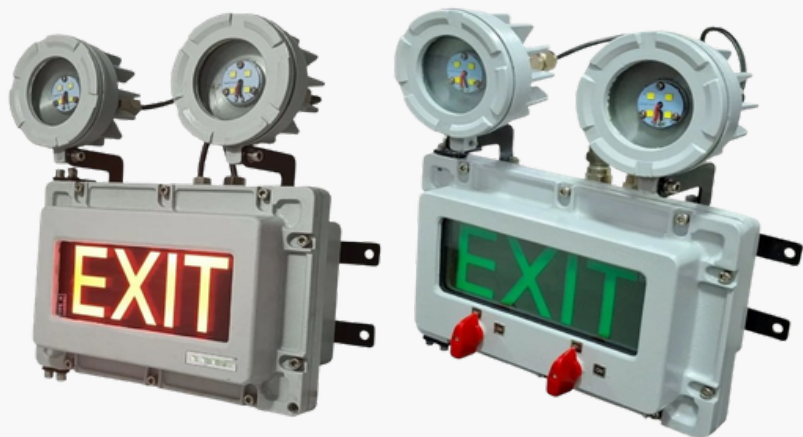
FLP LED Emergency Exit with Path Light Up to 40w
